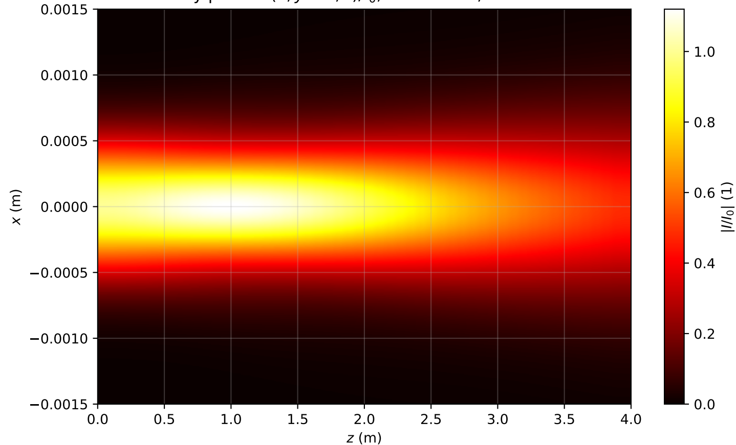
Intensity profile I(x, y = 0, z)/I_0 , P_{in}=0.6P_{cr} , artificial time
